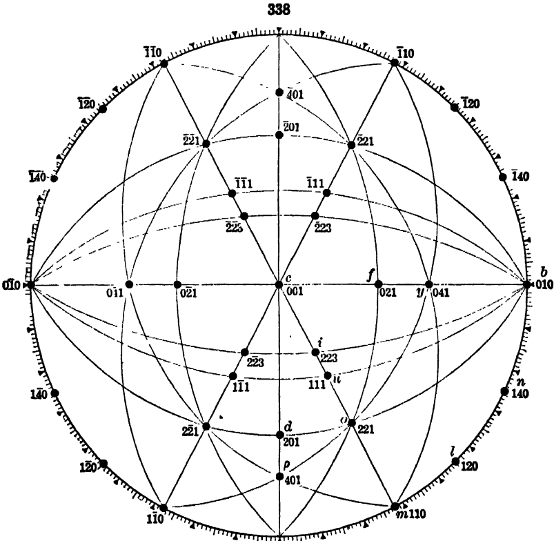
Stereographic Projection Topaz Crystal
